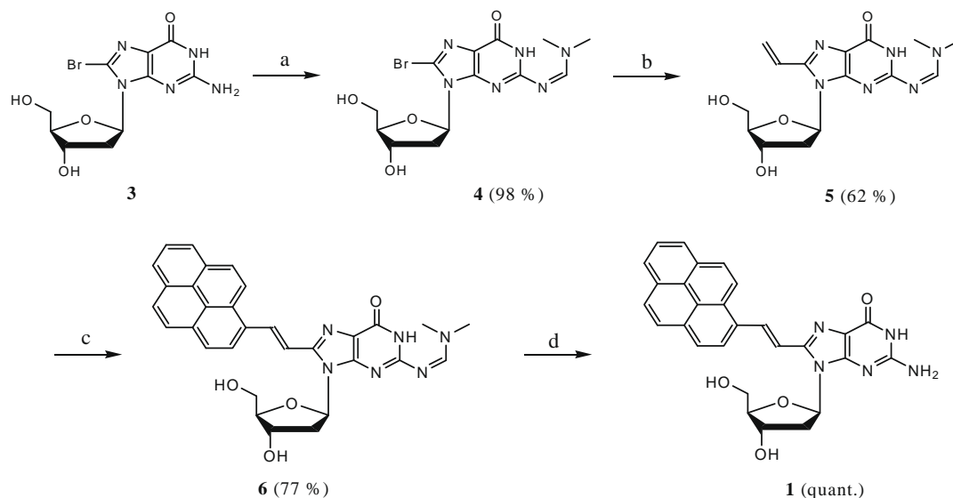
Scheme 1. Synthesis of photochromic nucleoside VPyG . Reagent and conditions: (a) DMF diethylacetal, methanol, 60 °C, 3 h; (b) Pd(PPh 3 ) 4 , Sn(CH 2 CH 2 ) 4 , Et 3 N, DMF, 60 °C, 12 h; (c) 1-bromopyrene, Pd(PPh 3 ) 4 , CH 3 COONa, DMF, 80 °C, 12 h; (d) NH 4 OH/methanol, rt, 8 h.
